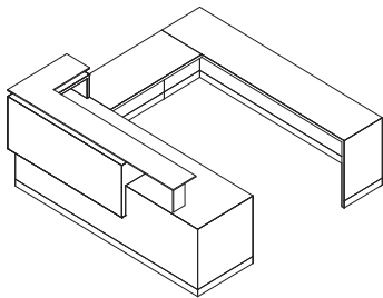
Desk, 48" w x 24" d bridge, and 20" d rear credenza shell, with three grommets. Specify left or right return.
